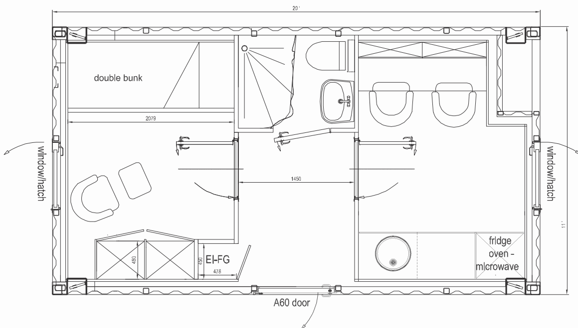
TITAN OFFSHORE MODULE 20 ( 20' x 11'x 10') 2 men sleeper/office/kitchenette - 6020 kg
