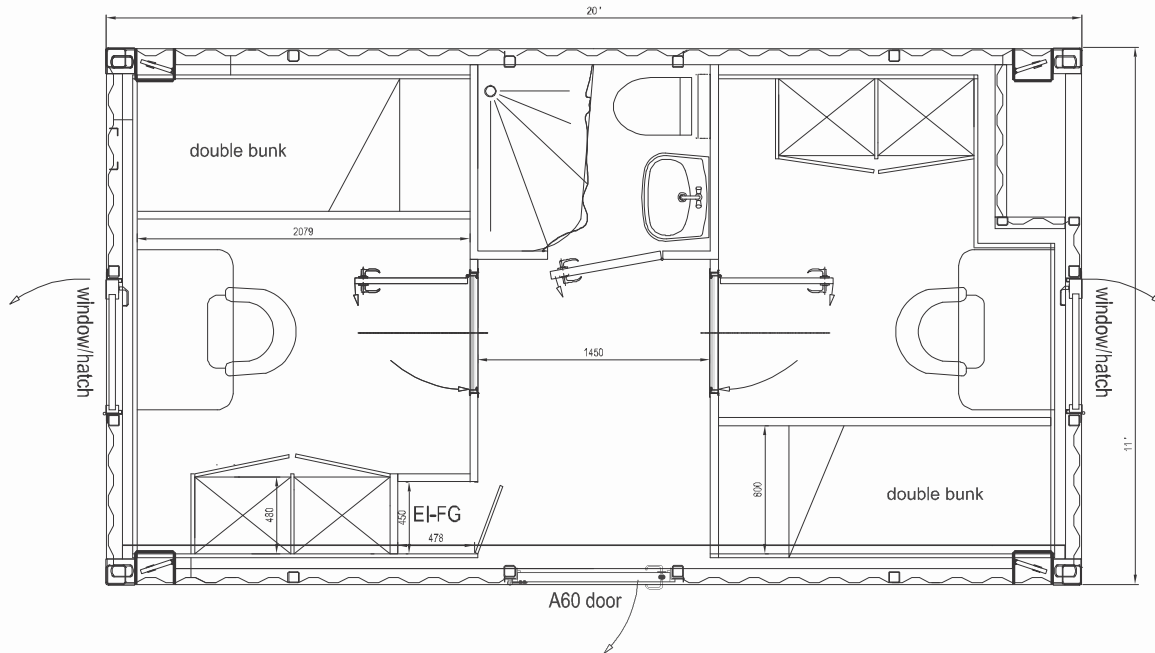
TITAN OFFSHORE MODULE 20 ( 20' x 11'x 10') 4 men sleeper - 5900 kg
